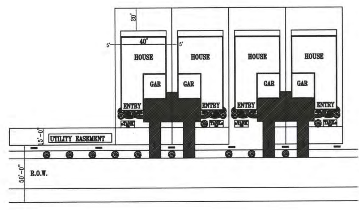
TYPICAL LOT & DRIVEWAY LAYOUT SCALE: NTS
